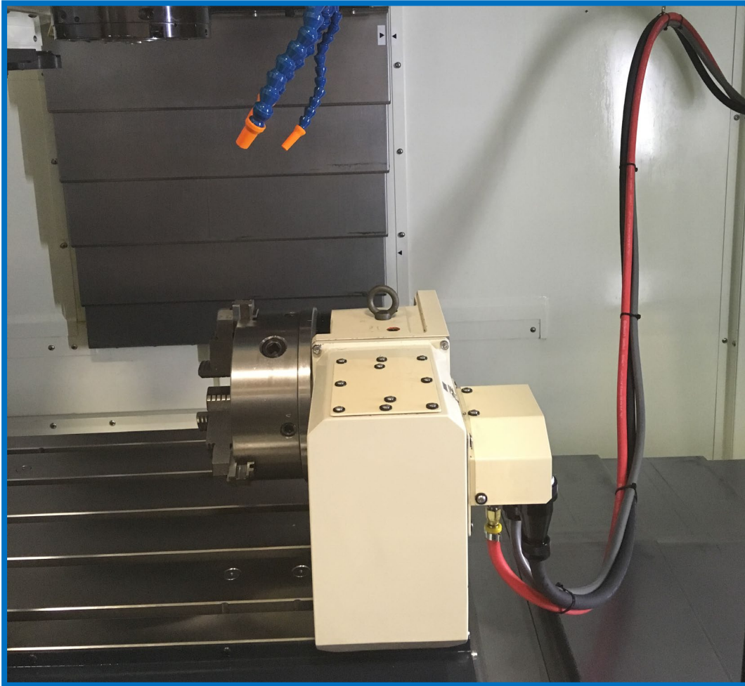
Tsudakoma RWA-200R, M (3-jaw chuck) 4 th axis installation on a Makino PS105 (VMC) with the PRO P control
