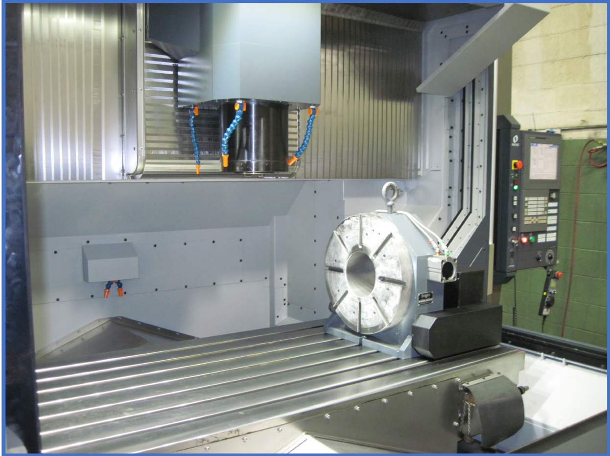
Troyke DL-16.5-B-RH-PC-O-180 4 th axis installation on a Makino F9 (VMC) with the PRO 5 control
