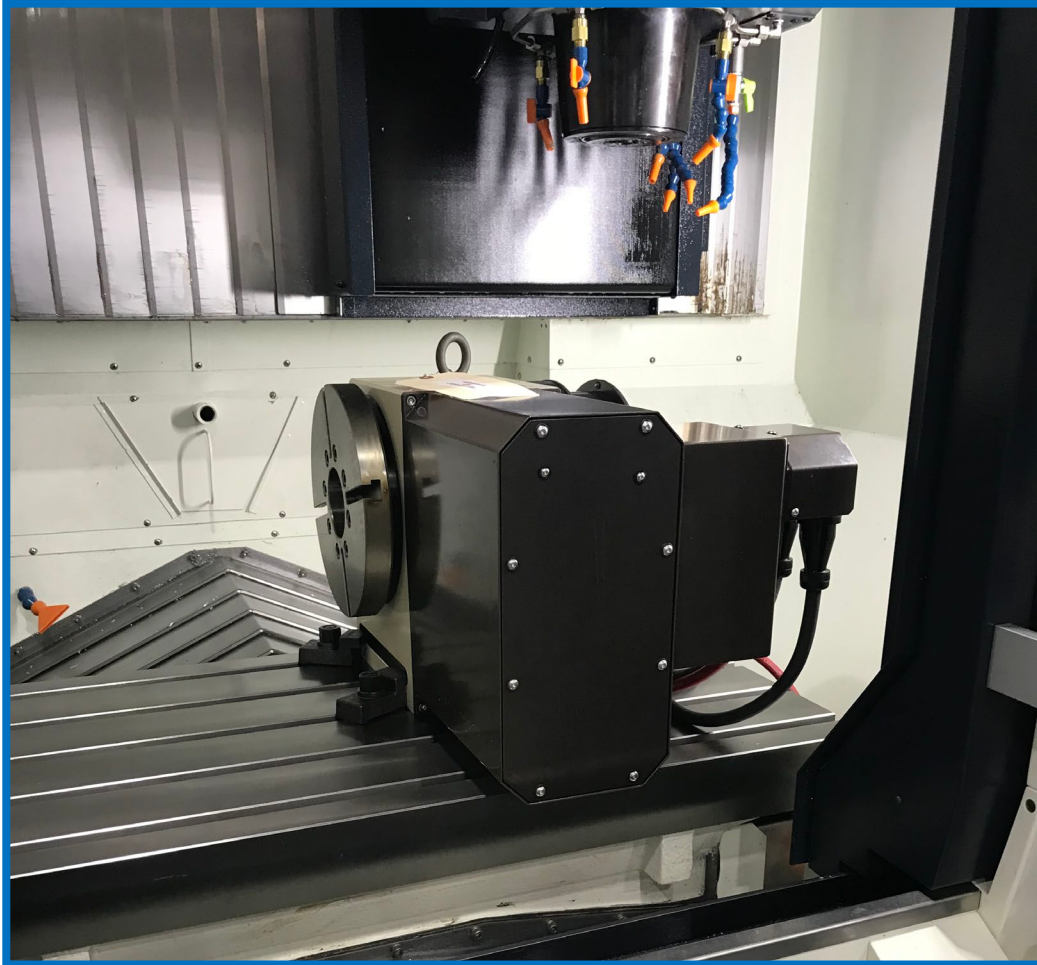
Tsudakoma RBS-250R, M 4 th axis installation on a Makino F5 (VMC) with the PRO 6 control
